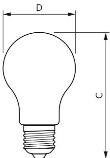
Bulb A67 100W 152lm 4000K E27 ND Clear
