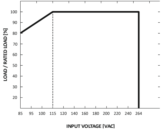
© STATIC CHARACTERISTIC
