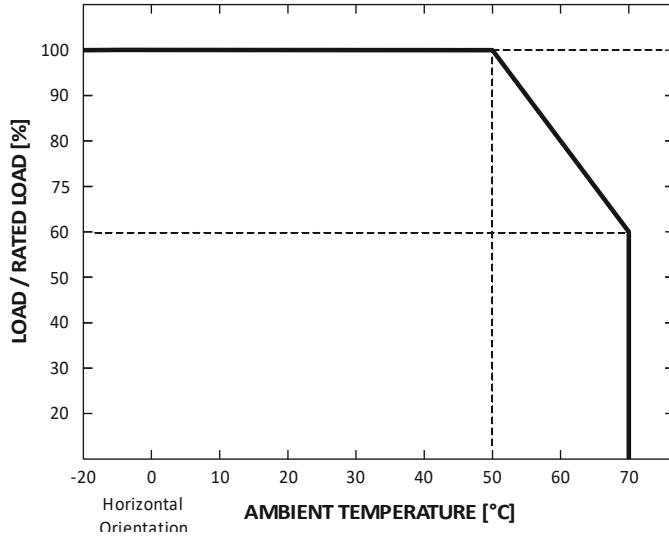
© DERATING CURVE
