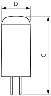
Capsule G4 1.9W-20W 200lm 2700K Non-Dim
