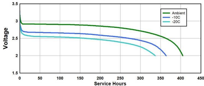
Cold Temperature Performance 5 kOhm Continuous to 2.0V
