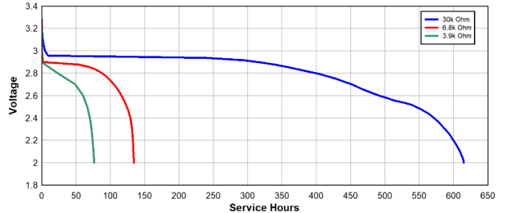
Continuous Discharge at Various Loads
